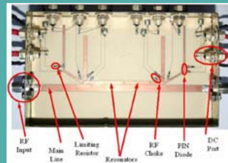
Fig.2 Filtro de microondas reconconfigurable
